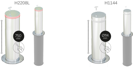
Semi-Automatic Telescopic with key and LED Ø220 x 500 SEMI-AUTOMATIC TELESCOPIC with key Ø114 x 500 mm
